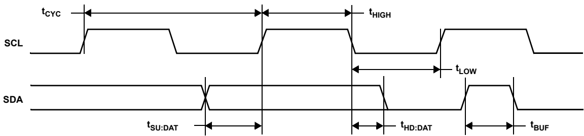
FIGURE 10. INPUT TIMING
