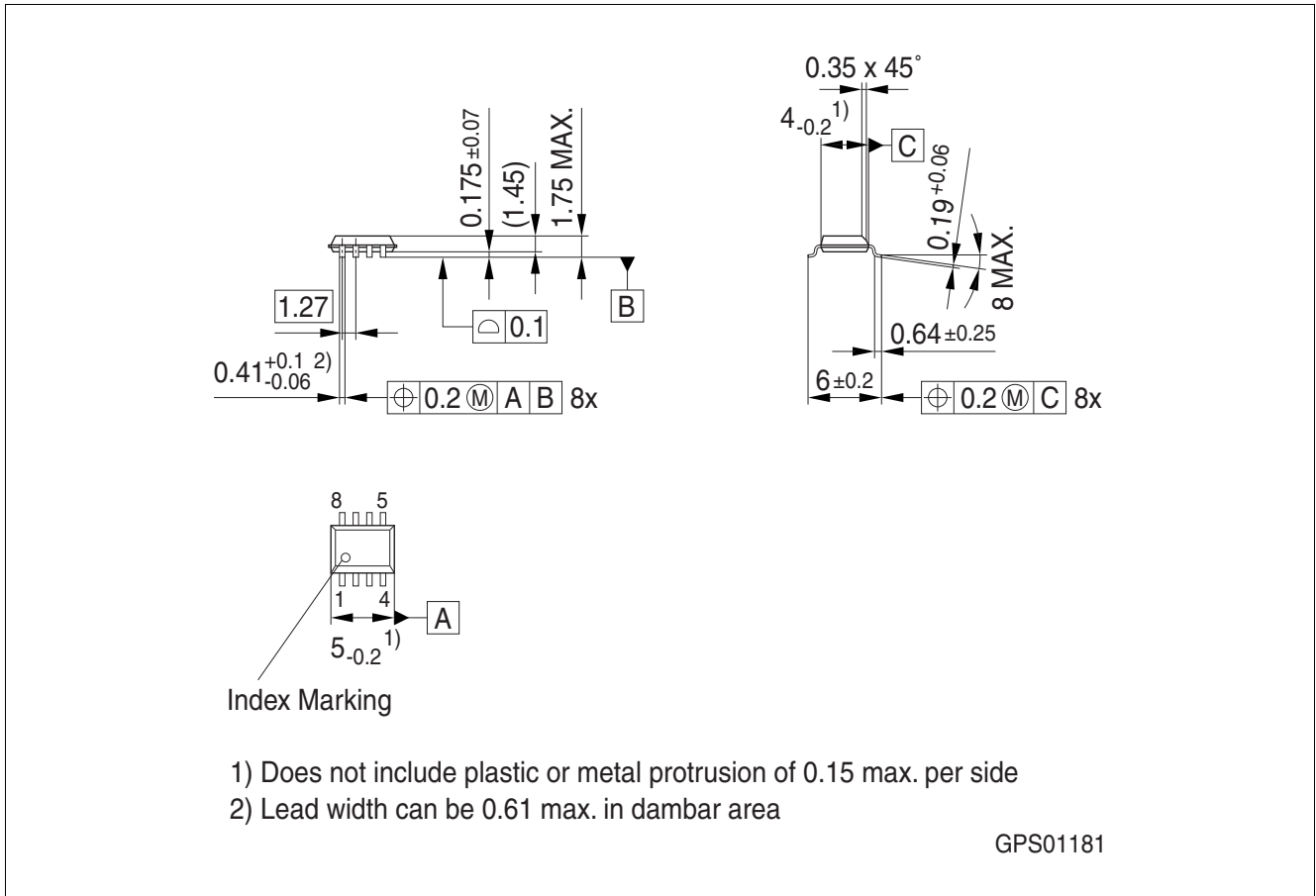
Figure 10 PG-DSO-8
