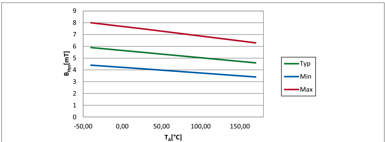
Figure 5-3 Hysteresis (B Hys ) of the TLE4964-2K over Temperature
