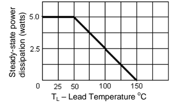
FIGURE 4 Steady-state power derating curve
