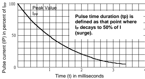
FIGURE 2 Pulse wave form for exponential surge
