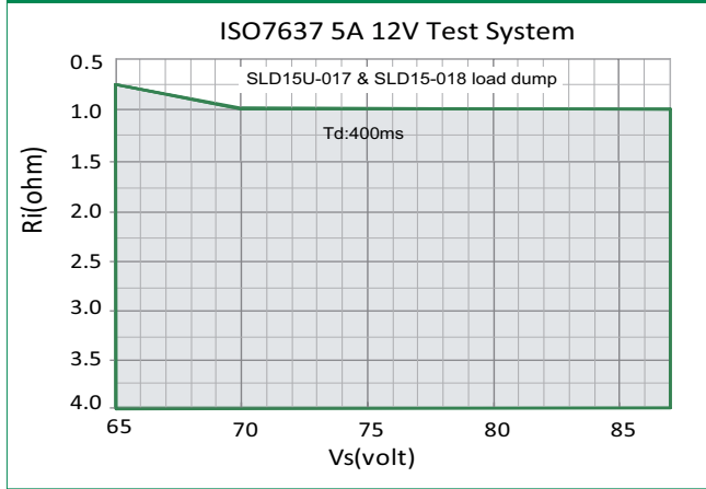
Figure 7 - SOA Chart
