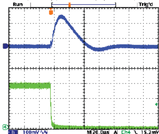
Step Load Transient Response (Vin=5.5V, Vout=3.3V, Cload=10x10µF X5R 0805 ceramic, plus 1x470µF, 7mΩ POSCAP, total 570µF, Iout=1.5A to 0A) Top trace=Vout, Bottom trace=Iout
