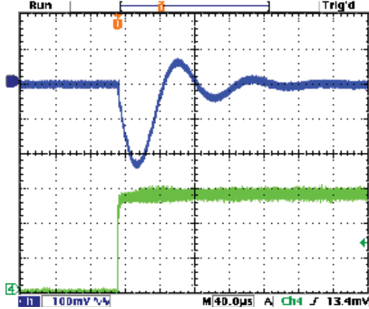
Step Load Transient Response (Vin=4.5V, Vout=1.8V, Cload=10x10µF X5R 0805 ceramic, plus 1x470µF, 7mΩ POSCAP, total 570µF, Iout=0A to 1.5A) Top trace=Vout, Bottom trace=Iout
