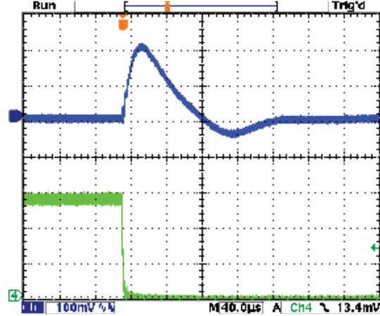
Step Load Transient Response (Vin=4.5V, Vout=1.8V, Cload=10x10µF X5R 0805 ceramic, plus 1x470µF, 7mΩ POSCAP, total 570µF, Iout=1.5A to 0A) Top trace=Vout, Bottom trace=Iout
