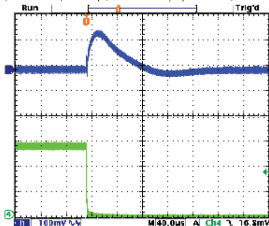
Step Load Transient Response (Vin=12V, Vout=3.3V, Cload=10x10µF 5R 0805 ceramic, plus 1x470µF, 7mΩ POSCAP, total 570µF, Iout=1.5A to 0A) Top trace=Vout, Bottom trace=Iout
