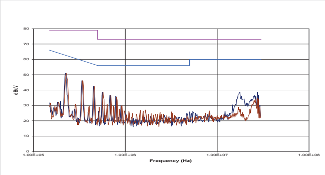
MTE1S0305MC
