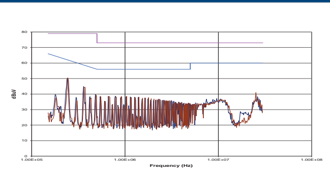
MTE1S0315MC
