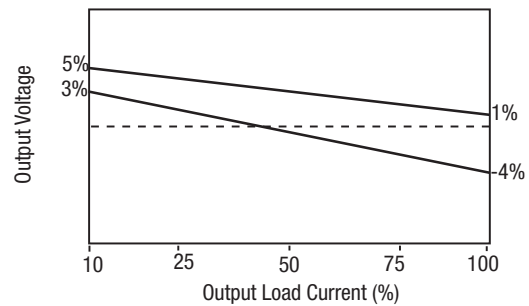
MGJ2D051505SC
