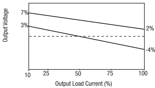
MGJ2D121509SC & MGJ2D241509SC
