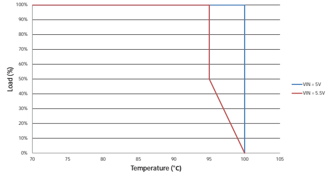
MGJ1D051510MPC
