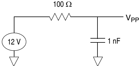
Figure 35. Example V PP Filtering
