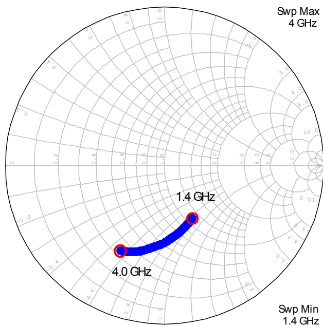
Output Return Loss
