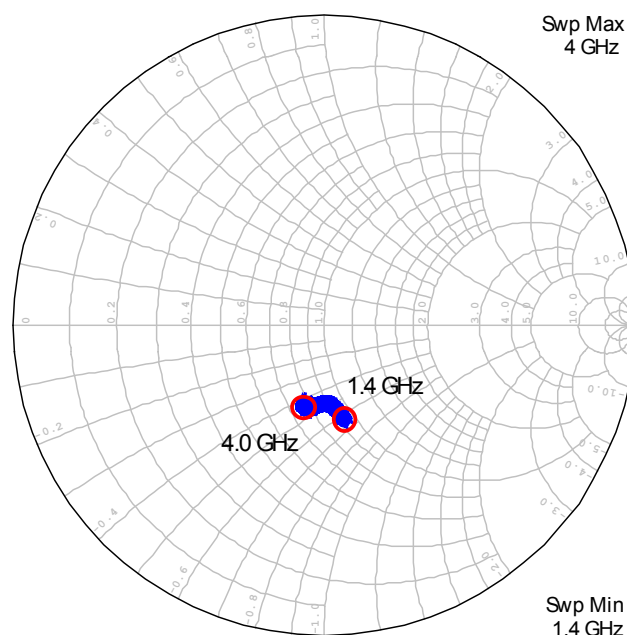
Input Return Loss
