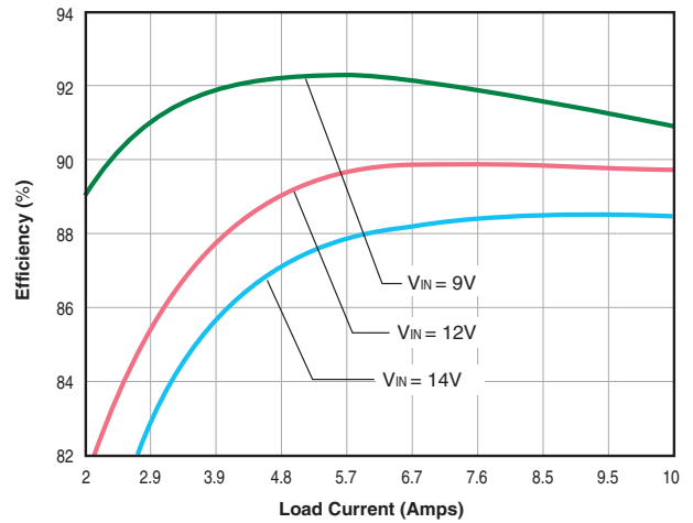
LSN-T/10-D12 Efficiency vs. Line Voltage and Load Current @ 25°C, Vout = 1.8V
