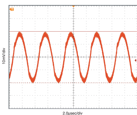
Output Ripple Noise (VIN = 12V, VOUT = 5V, IOUT = 10A, COUT = 10µF Tantalum || 1µF ceramic)
