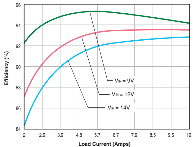
LSN-T/10-D12 Efficiency vs. Line Voltage and Load Current @ 25°C, Vout = 2.5V
