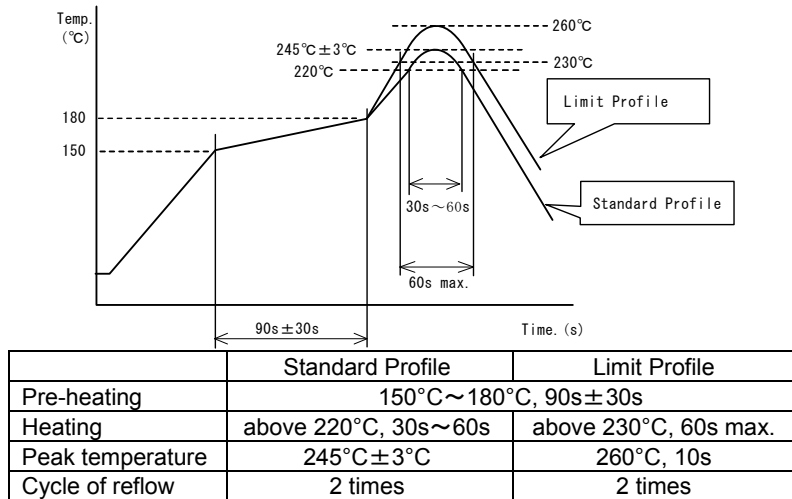
Soldering Profile for Lead Free solder
