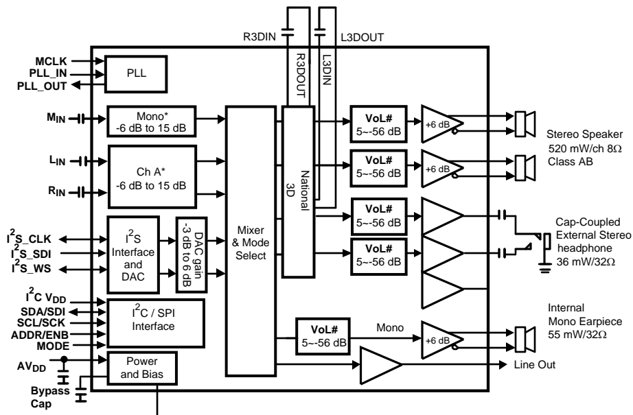
Figure 2. Audio Sub-System with SE HP Outputs
