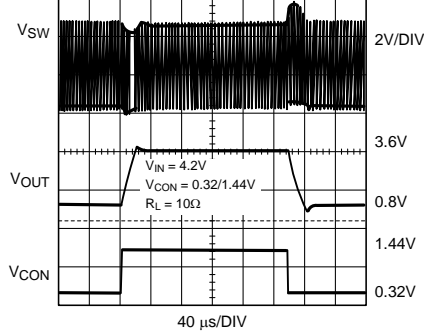
( V_{IN} = 4.2V, V_{CON} = 0.32V/1.44V, R_{LOAD} = 10\Omega )
