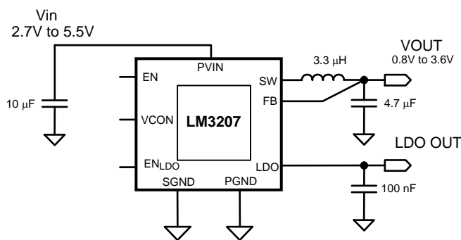
Figure 1. LM3207 Typical Application
