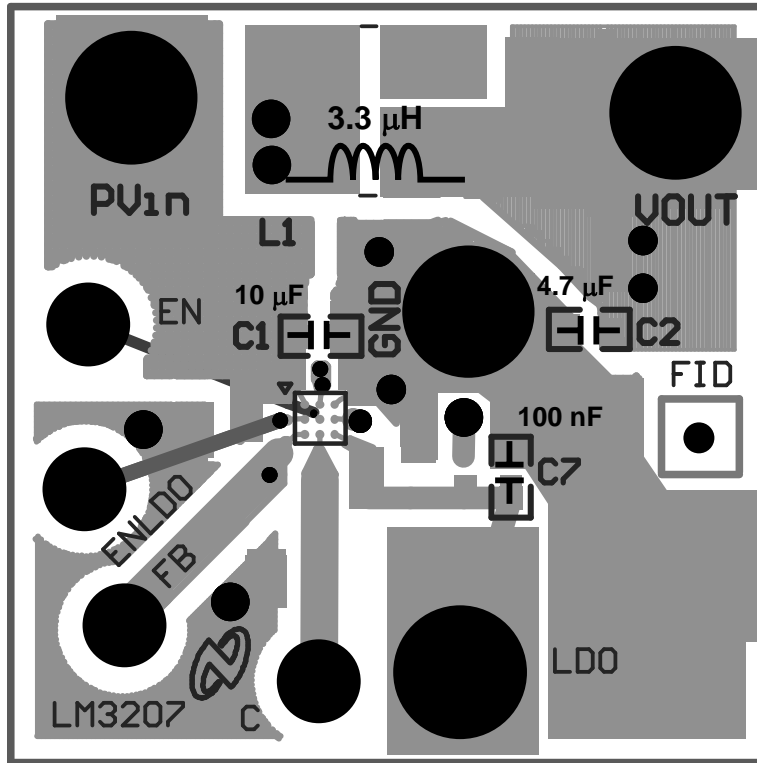
Figure 5. Evaluation Board Layout
