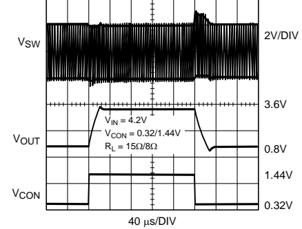
( V_{IN} = 4.2V, V_{CON} = 0.32V/1.44V, R_{LOAD} = 15\Omega/8\Omega )
