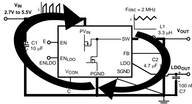
Figure 4. Current Loop
