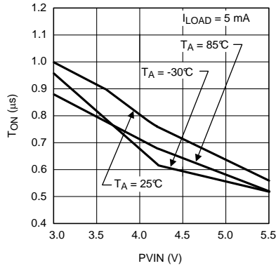
LDO Turn On Time vs V_{IN} ( C_{LDO} = 100nF )
