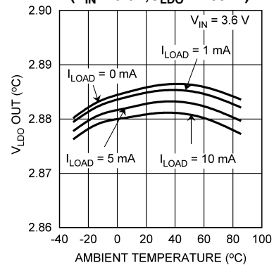
( V_{IN} = 3.6V , C_{LDO} = 100nF )
