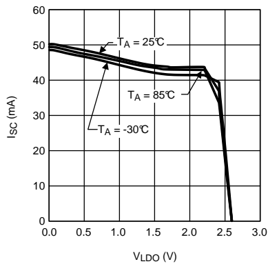
LDO Short Circuit Current vs Voltage ( V_{IN} = 3.0V , C_{LDO} = 100nF )
