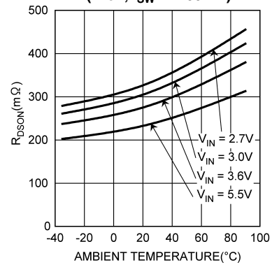
Temperature (microSMD) (N-ch, I_{SW} = -200mA )
