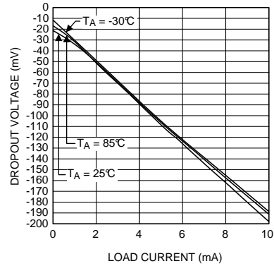
LDO Dropout Voltage vs Load Current ( C_{LDO} = 100nF ), (1)
