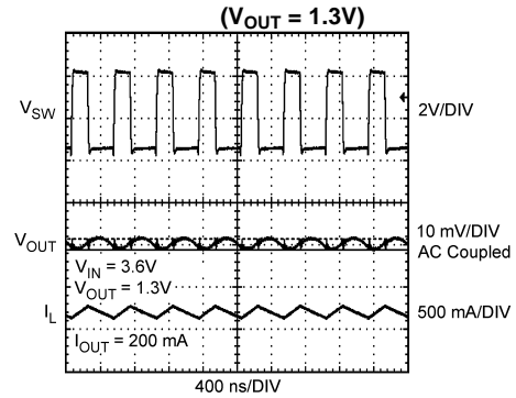
Output Voltage Ripple in Pulse Skip
