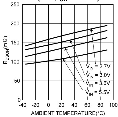
Temperature (microSMD) (P-ch, I_{SW} = 200mA )
