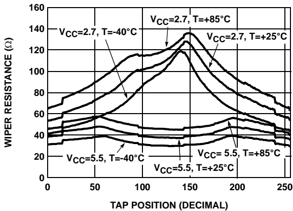
FIGURE 1. WIPER RESISTANCE vs TAP POSITION [I(RW) = V_{CC} / R_{TOTAL}] FOR 50k \Omega (U)
