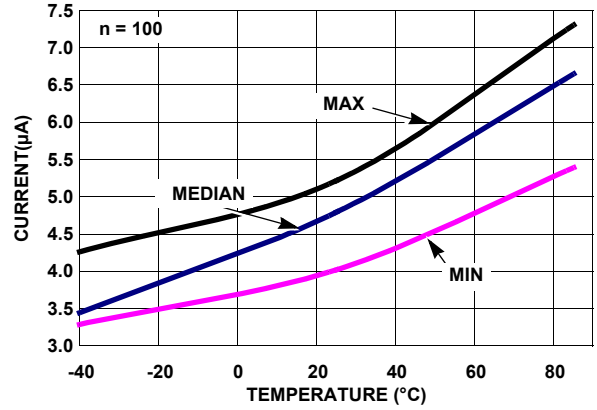
FIGURE 32. SUPPLY CURRENT DISABLED vs TEMPERATURE V_S = \pm 1.5V
