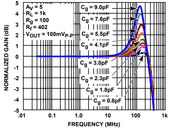
FIGURE 8. ISL5190 GAIN vs FREQUENCY vs C_g
