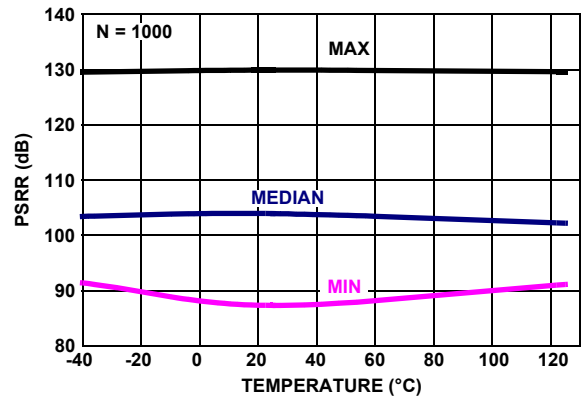
FIGURE 30. PSRR vs TEMPERATURE, V_+, V_- = \pm 1.2V \text{ TO } \pm 2.5V
