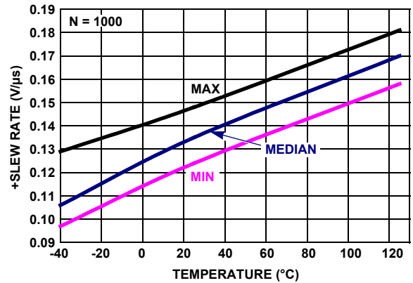
FIGURE 37. +SLEW RATE vs TEMPERATURE, V_{OUT} = \pm 1.5V, A_v = +2
