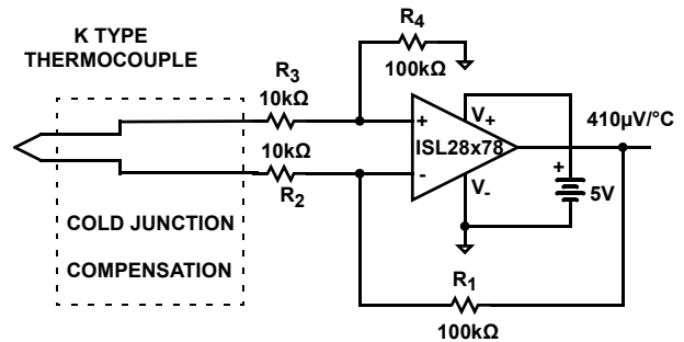
FIGURE 41. THERMOCOUPLE AMPLIFIER
