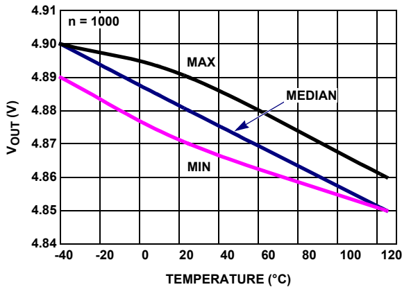
FIGURE 45. V_{OUT \text{ HIGH}} vs TEMPERATURE, R_L = 1k, V_+, V_- = \pm 2.5V
