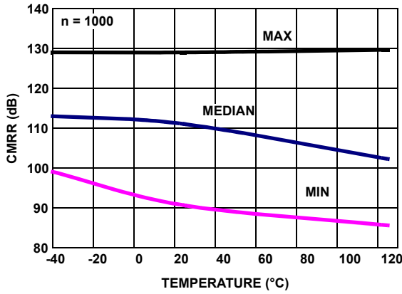
FIGURE 41. CMRR vs TEMPERATURE, V_{CM} = +2.5V \text{ TO } -2.5V, V_+, V_- = \pm 2.5V
