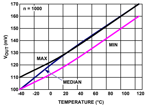
FIGURE 46. V_{OUT \text{ LOW}} vs TEMPERATURE, R_L = 1k, V_+, V_- = \pm 2.5V
