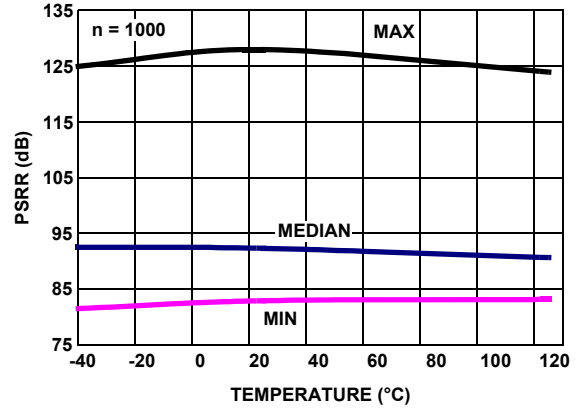
FIGURE 42. PSRR vs TEMPERATURE, V_+, V_- = \pm 1.2V \text{ TO } \pm 2.5V
