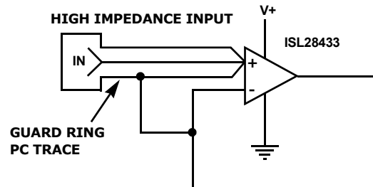
FIGURE 43. USE OF GUARD RINGS TO REDUCE PARASITIC CAPACITANCE
