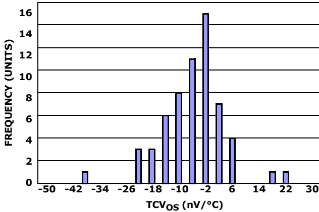
FIGURE 36. TCV_{OS} HISTOGRAM
