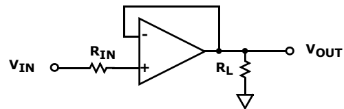
FIGURE 42. INPUT CURRENT LIMITING
