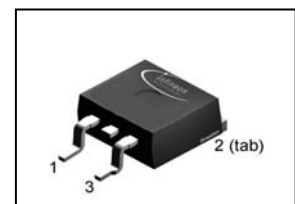
PG-TO263-3
