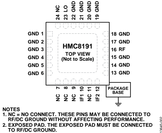
Figure 2. Pin Configuration
