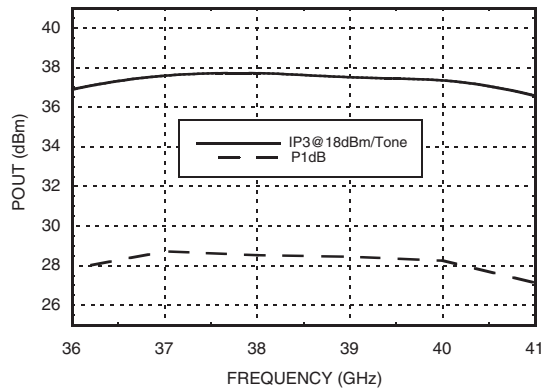
Fixtured Power vs. Frequency
