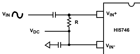
FIGURE 28. AC COUPLED SINGLE ENDED INPUT
