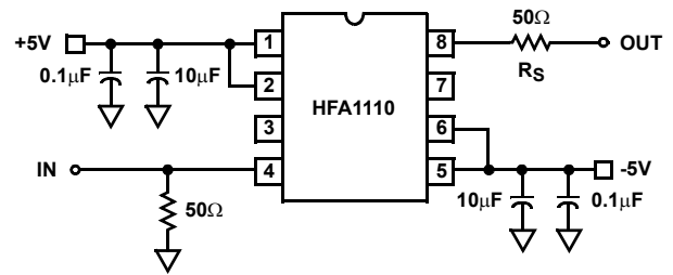
SCHEMATIC DIAGRAM
