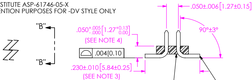
FIG 2 FTS-1XX-03-XX-DV SHOWN (DIFFERENT AS SHOWN, OTHERWISE SAME AS FIG 1)
