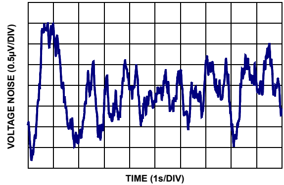
FIGURE 16. EL8173 0.1Hz TO 10Hz INPUT VOLTAGE NOISE (GAIN = 10)
