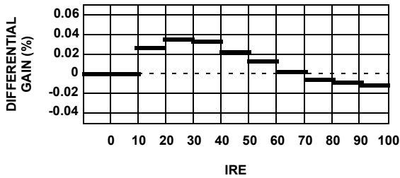
FIGURE 35. DIFFERENTIAL GAIN
