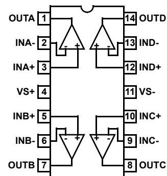
EL5451 (14 LD SOIC) TOP VIEW
