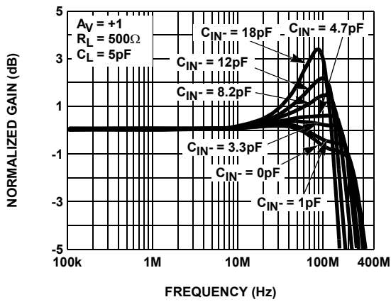
FIGURE 9. EL5150 GAIN vs FREQUENCY FOR VARIOUS C_{IN}
