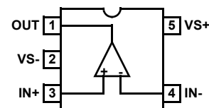
EL5151 (5 LD SOT-23) TOP VIEW
