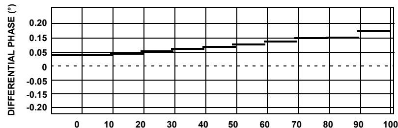
FIGURE 36. DIFFERENTIAL PHASE (°)
