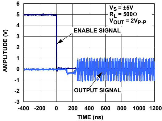
FIGURE 25. ENABLE TIME
