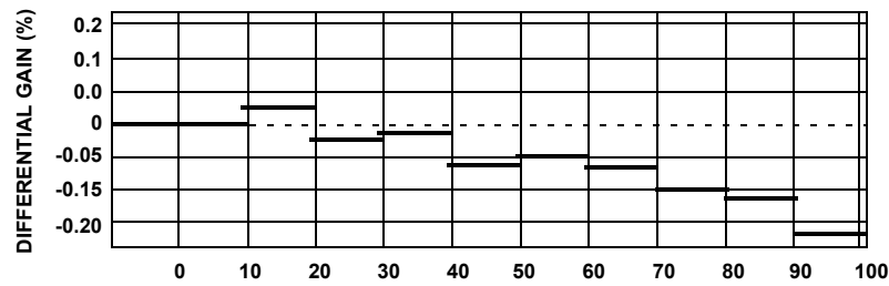
FIGURE 35. DIFFERENTIAL GAIN (%)
