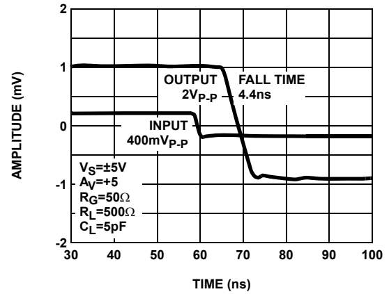
FIGURE 32. LARGE SIGNAL PULSE RESPONSE/FALL TIME
