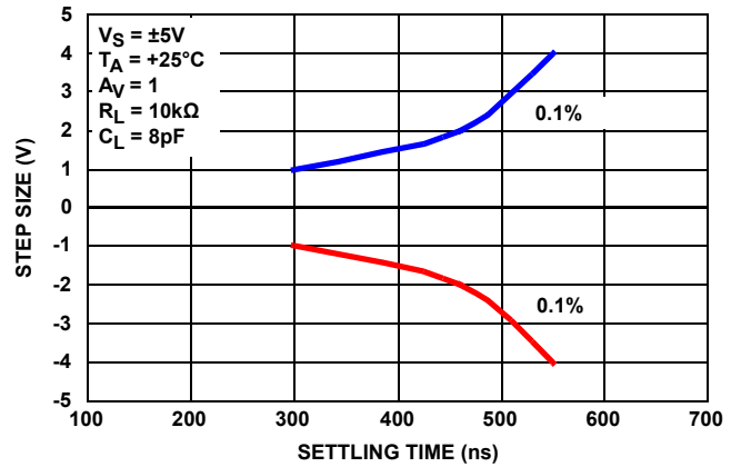
FIGURE 24. STEP SIZE vs SETTLING TIME
