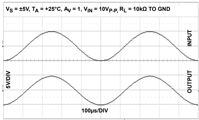
FIGURE 29. OPERATION WITH RAIL-TO-RAIL INPUT AND OUTPUT
