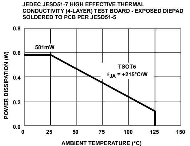
FIGURE 31. PACKAGE POWER DISSIPATION vs AMBIENT TEMPERATURE
