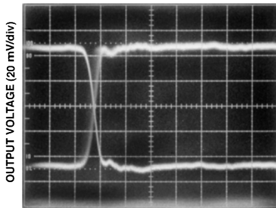
Small-Signal Step Response
