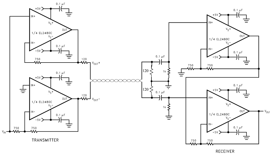
DIFFERENTIAL LINE-DRIVER/RECEIVER
