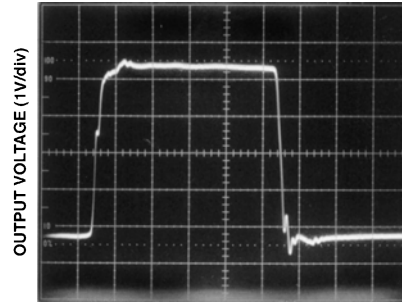
Large-Signal Step Response
