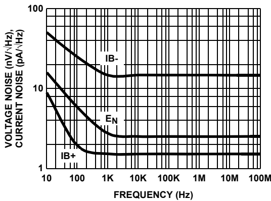
FIGURE 11. VOLTAGE AND CURRENT NOISE vs FREQUENCY
