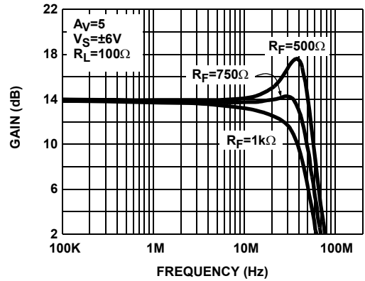
FIGURE 2. DIFFERENTIAL FREQUENCY RESPONSE vs R_F
