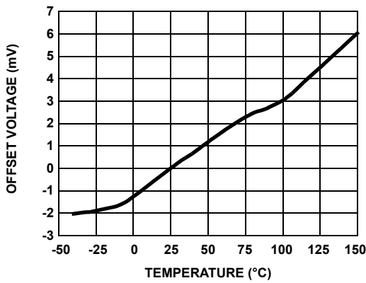
FIGURE 21. OFFSET VOLTAGE vs TEMPERATURE
