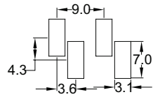
Recommended Pad Layout
