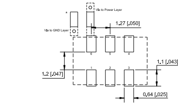
Recommended Land Pattern for LVPECL, LVDS, HCSSL
