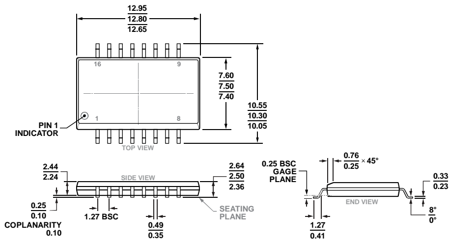
Figure 25. 16-Lead Standard Small Outline Package [SOIC_W] Wide Body (RW-16) Dimensions shown in millimeters and (inches)
