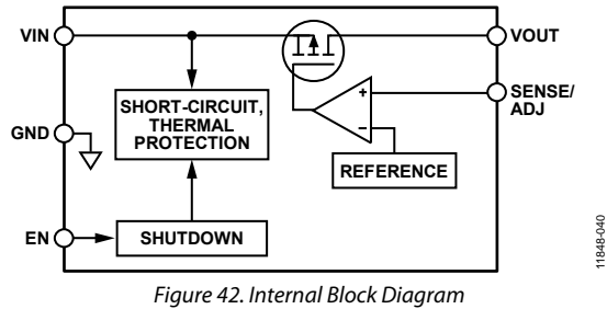
Figure 42. Internal Block Diagram
