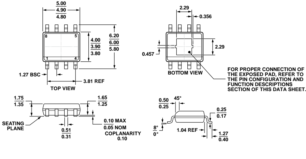
COMPLIANT TO JEDEC STANDARDS MS-012-AA Figure 68. 8-Lead Standard Small Outline Package, with Exposed Pad [SOIC_N_EP] Narrow Body (RD-8-1) Dimensions shown in millimeters
