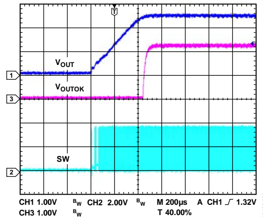
Figure 33. VOUTOK Function
