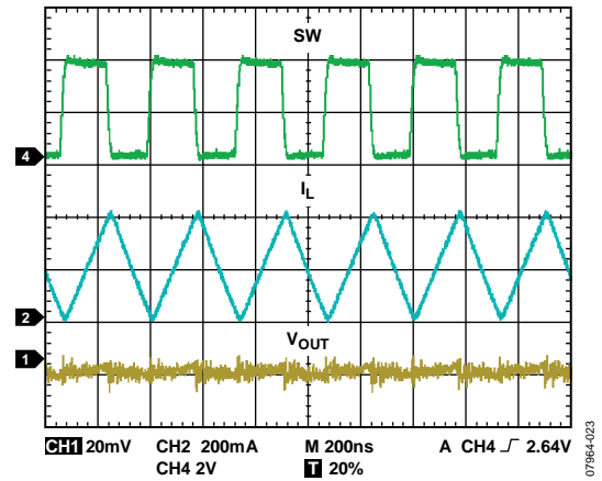
Figure 24. Typical PWM Waveform, 200\text{ mA}
