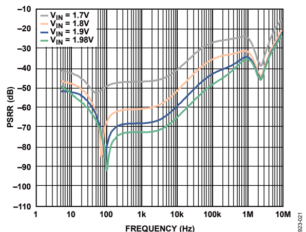
Figure 21. Power Supply Rejection Ratio (PSRR) vs. Frequency for Various Input Voltages, V_{OUT} = 1.5\text{ V} , Load Current = 3 A
