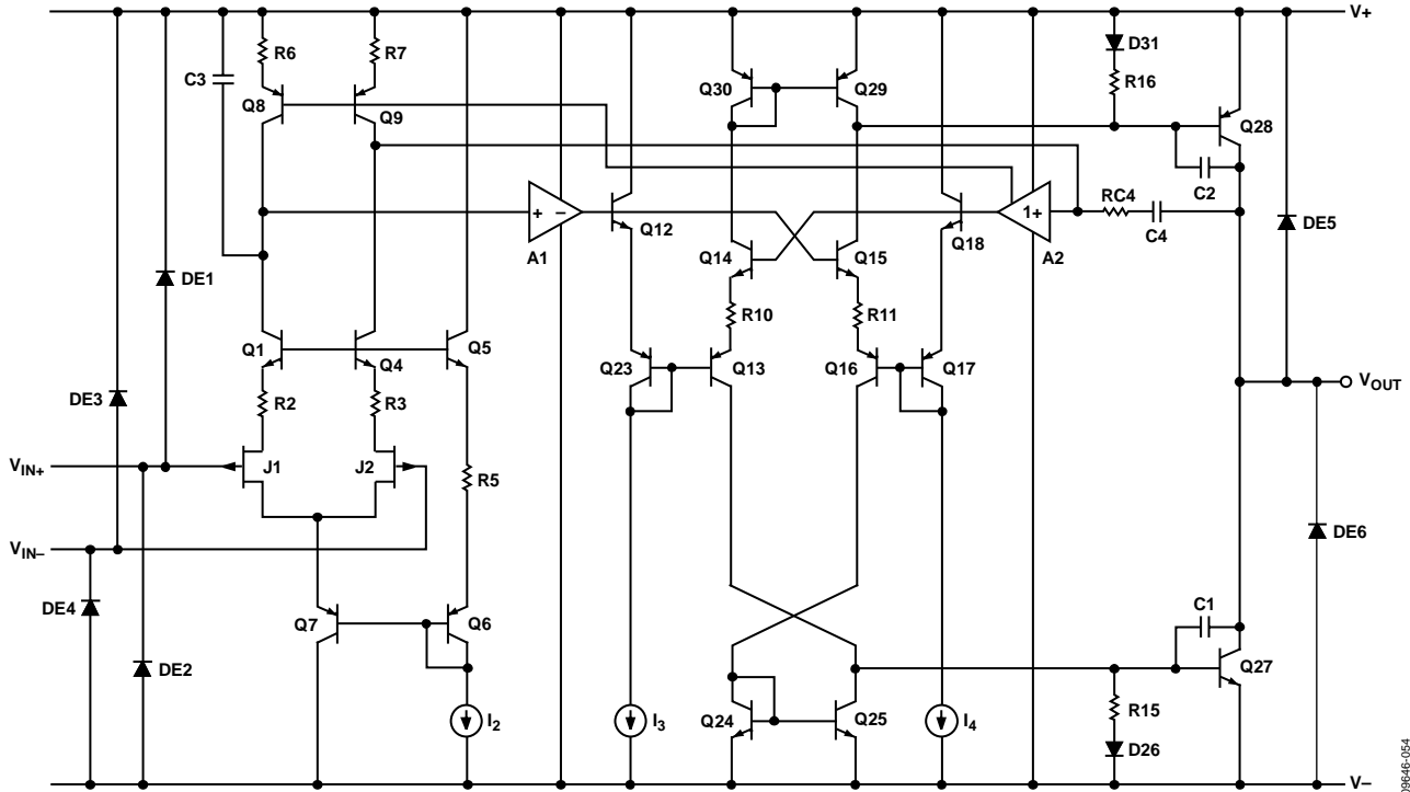
Figure 57. Simplified Schematic
