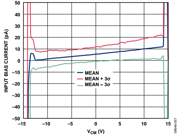
Figure 18. Input Bias Current vs. Common-Mode Input Voltage ( V_{CM} ), Mean and Three Standard Deviations, V_{SY} = \pm 15 V, R_L = \infty
