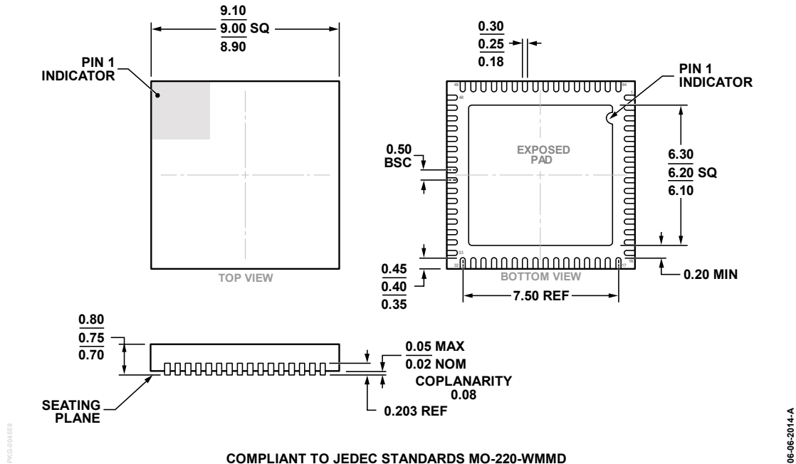
COMPLIANT TO JEDEC STANDARDS MO-220-WMMD Figure 44. 64-Lead Lead Frame Chip Scale Package [LFCS] 9 mm × 9 mm and 0.75 mm Package Height (CP-64-17) Dimensions shown in millimeters
