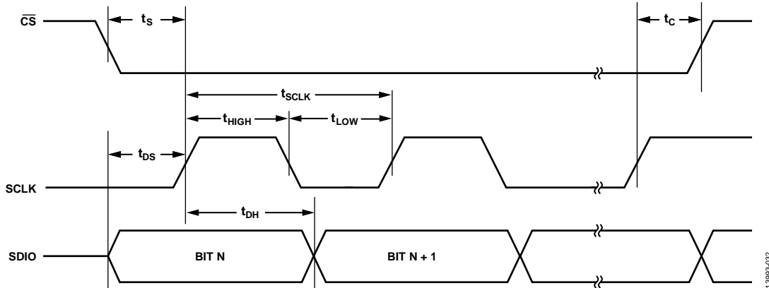
Figure 32. Timing Diagram for Serial Control Port—Write
