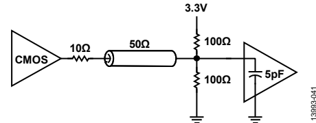
Figure 41. CMOS Output with Far End Termination
