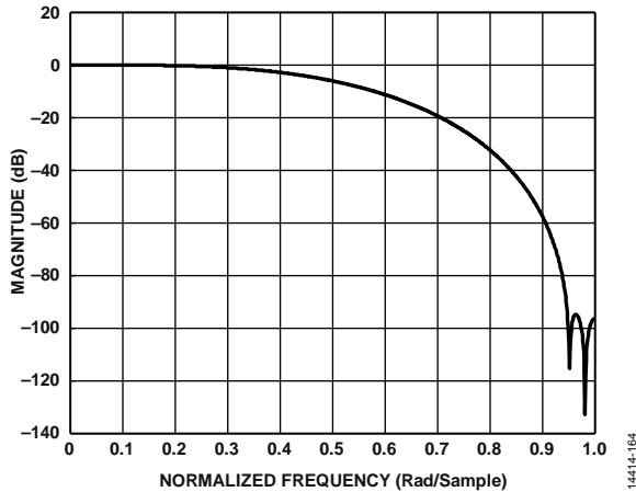
Figure 118. Fourth 2x Half-Band 11.25% Filter Response
