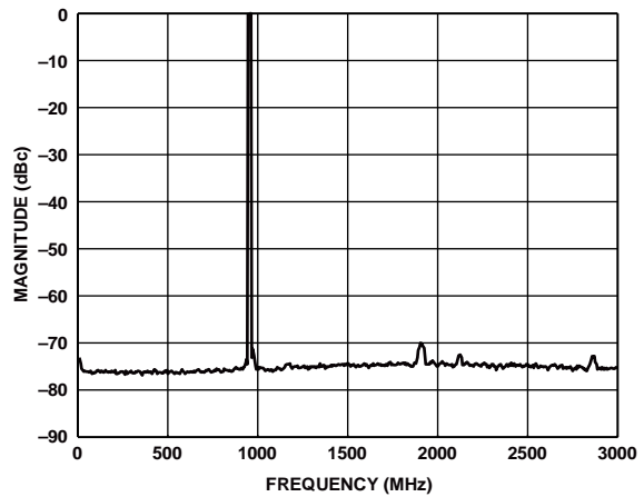
Figure 70. Four Carriers at 950 MHz Output (Shuffle On)
