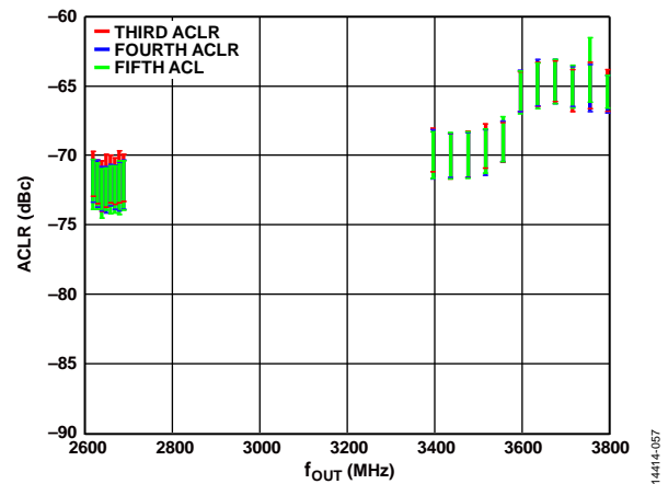
Figure 59. Four-Carrier, W-CDMA ACLR vs. f_{OUT} (Third ACLR, Fourth ACLR, Fifth ACLR)
