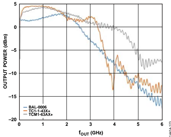
Figure 139. Measured DAC Output Response; f_{DAC} = 6 GSPS
