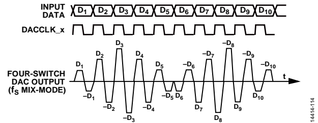
Figure 130. Mix-Mode Waveform
