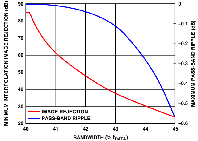
Figure 111. Interpolation Filter Performance Beyond Specified Bandwidth for the 80% Filters
