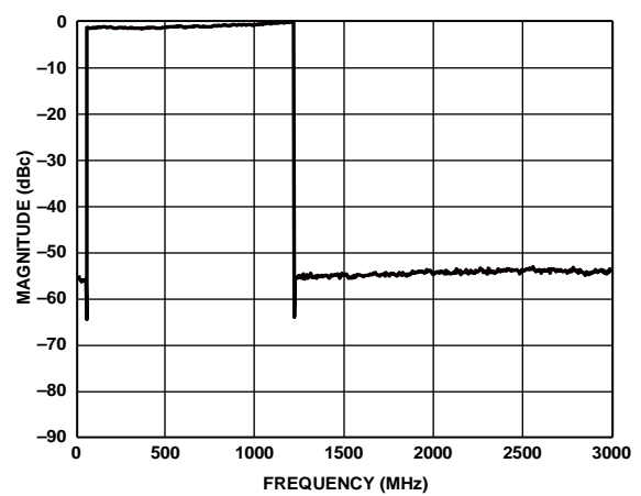
Figure 82. 194-Carrier, Sinc Enabled, FIR85 Enabled
