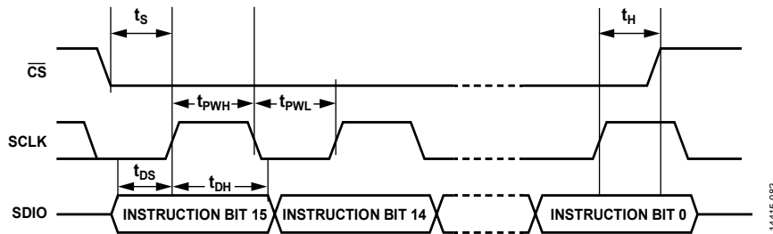
Figure 89. Timing Diagram for Serial Port Register Write
