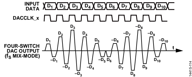
Figure 128. Mix-Mode Waveform
