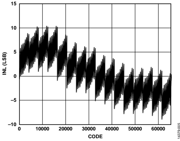
Figure 58. INL, I_{OUTFS} = 20\text{ mA}
