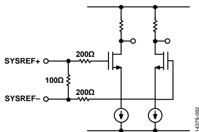
Figure 152. SYSREF± Input Circuit for the 8 mm x 8 mm 165-Ball BGA
