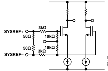
Figure 153. SYSREF± Input Circuit for the 11 mm x 11 mm 169-Ball BGA
