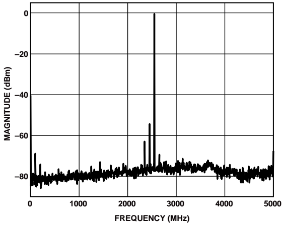
Figure 95. Single-Tone Spectrum at f_{OUT} = 2350\text{ MHz} (FIR85 Enabled)
