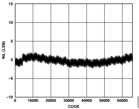
Figure 60. INL, I_{OUTFS} = 40\text{ mA}
