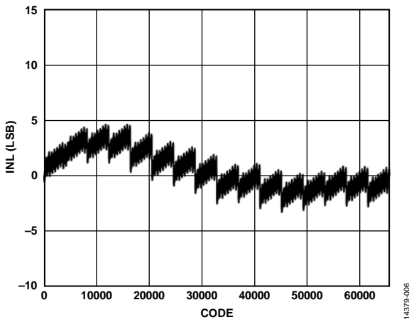
Figure 59. INL, I_{OUTFS} = 30\text{ mA}
