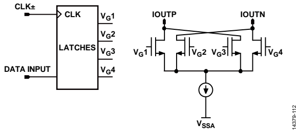
Figure 180. Quad-Switch Architecture
