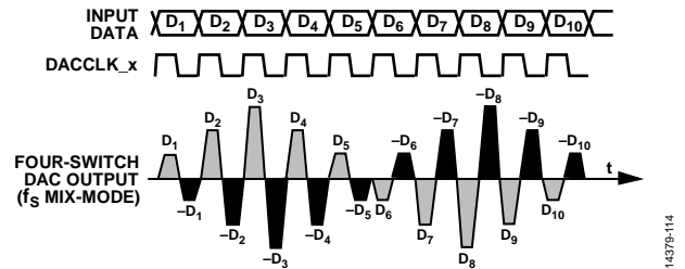
Figure 182. Mix-Mode Waveform
