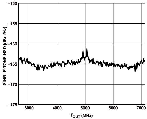
Figure 96. Single-Tone NSD vs. f_{OUT}
