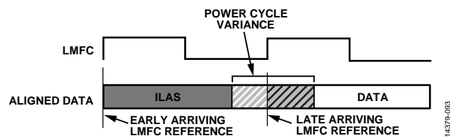
Figure 155. Link Delay > LMFC Period Example
