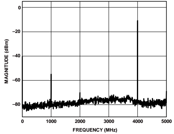
Figure 98. Single-Tone Spectrum at f_{OUT} = 4000\text{ MHz} (FIR85 Enabled)
