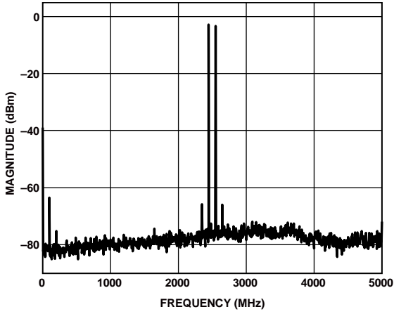
Figure 94. Single-Tone Spectrum at f_{OUT} = 2350\text{ MHz}
