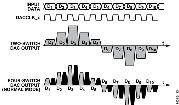
Figure 181. Two-Switch and Quad-Switch DAC Waveforms
