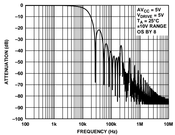
Figure 55. Digital Filter Response for OS x 8
