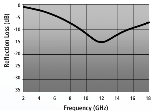
Typical electrical performance
