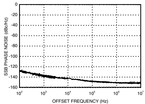
Residual Phase Noise Performance, P_{in} = 0\text{ dBm}, T = 25\text{ }^{\circ}\text{C}
