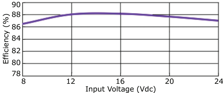
VX078012-500 Efficiency Curve Negative Output, Efficiency vs. Input Voltage (at full load)
